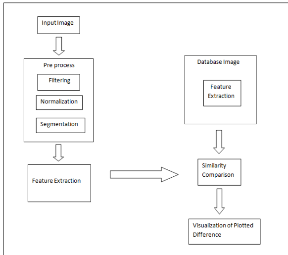
Figure1: Architecture for Fraud Detection based Online Test [FDOT] and Behavior identification through Visualization Techniques [BIVT]
