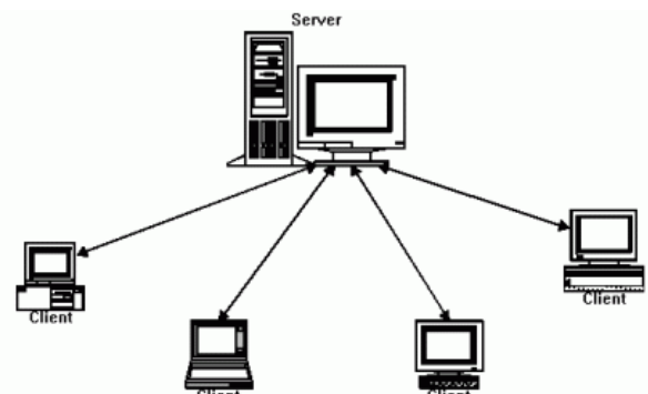
Fig. 1 Client-Server Architecture
