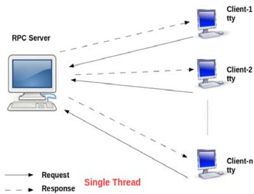
Fig. 6 Architecture of Online Examination System using Command Line Interface
