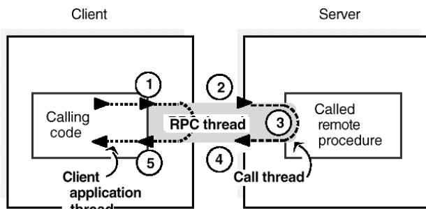
Fig. 2 Remote Procedure Call Structure
