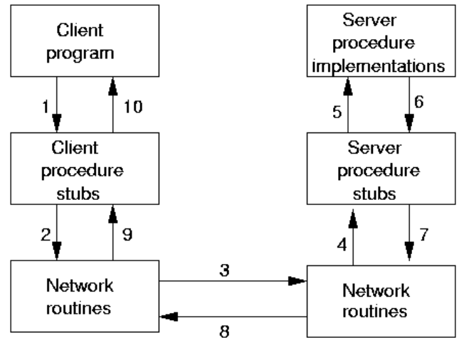
Fig.3 RPC Communication Structure
